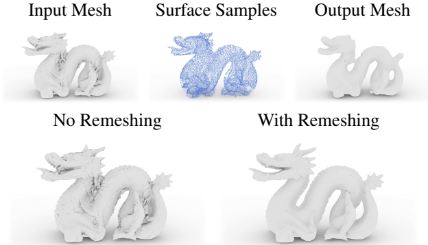
Figure 4. Effect of the remeshing step. (Left) A degraded mesh mid-optimization. (Middle) Point samples on the exterior surface. (Right) Poisson surface reconstruction on points. Artifacts disappear and fine detail can be recovered by subsequent optimization. The genus of the object changes from 0 to 1. (Bottom) Final outputs. Self-intersecting geometry degrades the reconstruction and hinders further optimization. Both optimizations are initialized as sphere clouds to emphasize behavior of this step.
