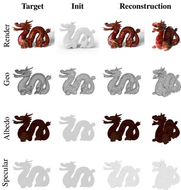
Figure 7. Reconstruction of the Stanford dragon inside a Cornell Box, with a glossy wood material. The image resolution was 128 \times 128 . Col. 2 shows initializations; Col. 4 shows a novel view. Although the geometry reconstruction exhibits dense triangle clusters, it is intersection-free: clusters are caused by our adaptive remeshing, which concentrates vertices in high detail areas. Re-renderings were produced using the Blender Cycles renderer..
